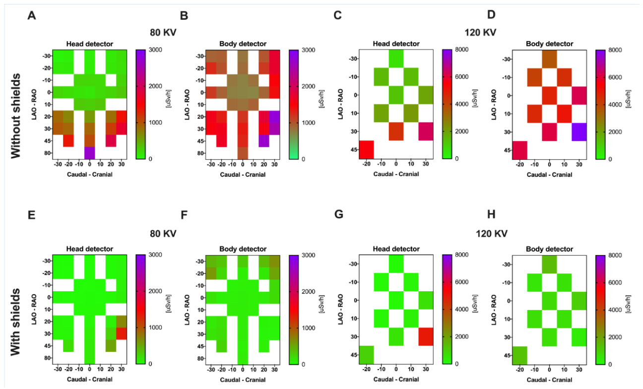
Supplementary Figure 3. Scattered radiation reduction performance at different catheterisation laboratory (CL) personnel positions (bench tests).
