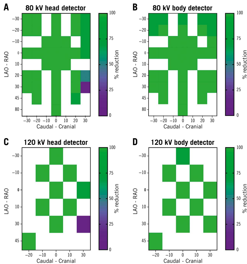
Figure 2. Scattered radiation reduction performance at different CL personnel positions (bench tests). The X-axis represents the C-arm angle in the caudal-cranial plane, the Y-axis represents the C-arm angle in the LAO-RAO plane. A, B) Percentage of radiation reduction (averaged) while using the radiation shields at 80 kV as depicted by the primary operator head detector (height of 155 cm from the floor) and body detector (height of 75 cm from the floor). The colour scale represents the percentage of radiation reduction in 0-25%, 25-50%, 50-75% and 75-100% categories. C, D) Percentage of radiation reduction while using the radiation shields at 120 kV as depicted by the primary operator head detector (height of 155 cm from the floor) and body detector (height of 75 cm from the floor). LAO: left anterior oblique; RAO: right anterior oblique
